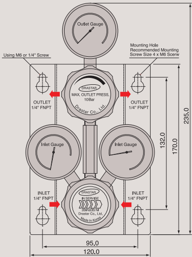
FUNCTIONAL SCHEMATIC
