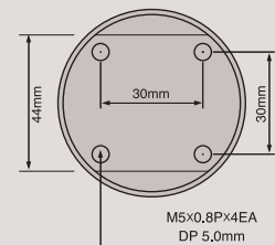
BRACKET CUT-OUTS
