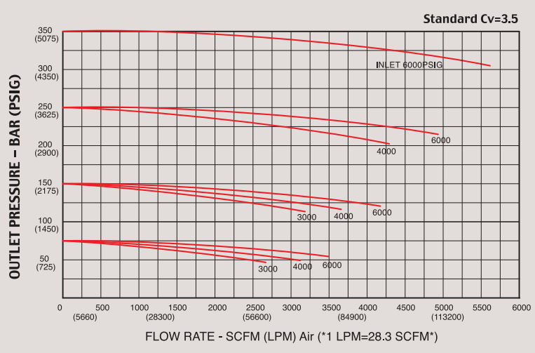
FLOW RATE L/Min AIR
