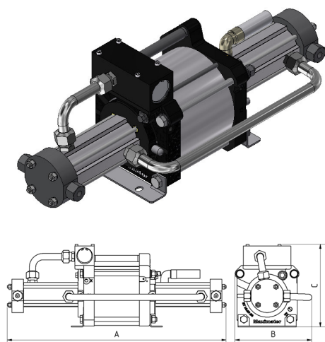
DLE 15 double acting, single air drive head single stage
