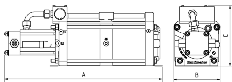
DLE 5-1-2 single acting, single air drive head single stage
