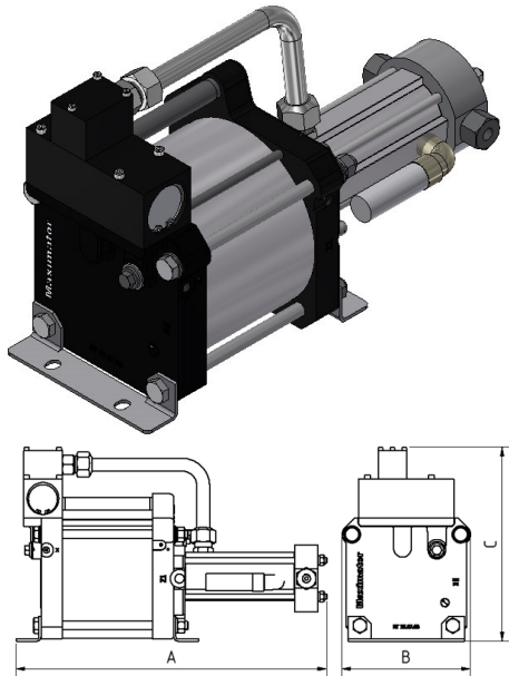
DLE 75-1 single acting, single air drive head single stage
